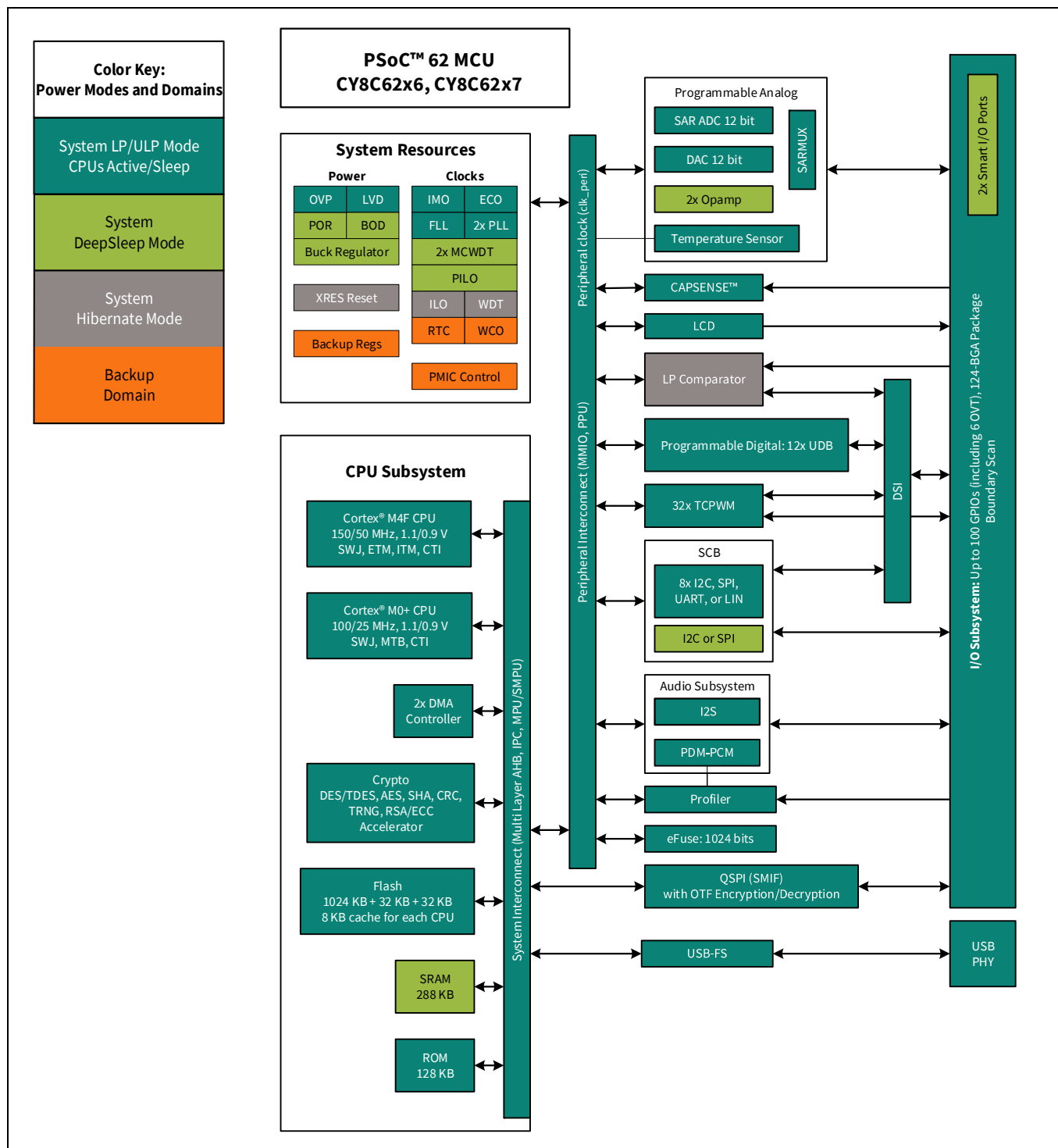
Figure 3 Block diagram
