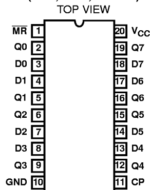
CD54HC273, CD54HCT273, CD74HC273, CD74HCT273 (PDIP, SOIC, Cerdip)
