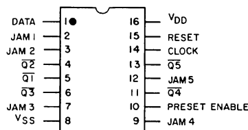
TERMINAL DIAGRAM Top View
