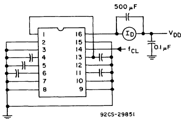
Fig. 14 – Dynamic power dissipation test circuit.
