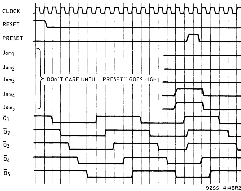
Fig. 15 — Timing diagram.
