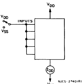
Fig. 11 – Quiescent device current test circuit.
