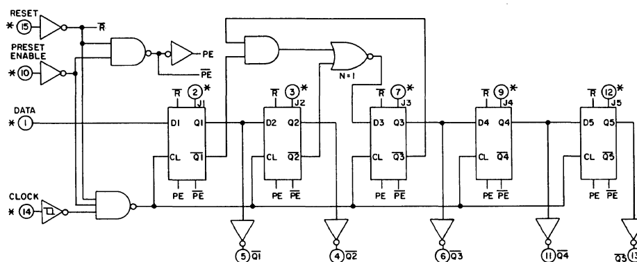
Fig. 1 — Logic diagram.
