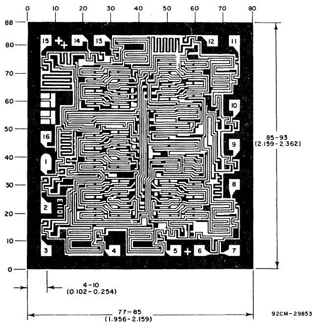
Dimensions and pad layout for CD4018B.
