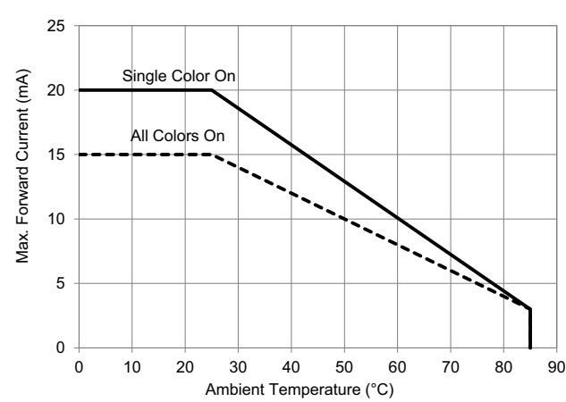
Figure 5: Derating Curve
