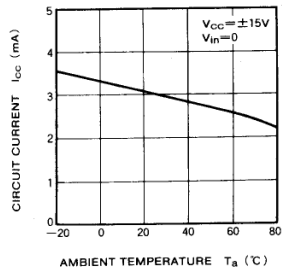
CIRCUIT CURRENT VS. AMBIENT TEMPERATURE
