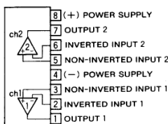
Outline 8P5 (AL)
