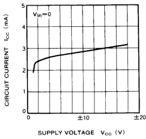
CIRCUIT CURRENT VS. SUPPLY VOLTAGE
