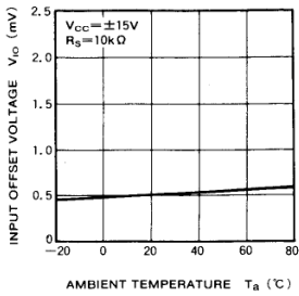
INPUT OFFSET VOLTAGE VS. AMBIENT TEMPERATURE
