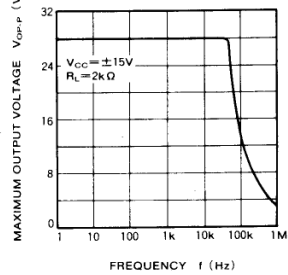
MAXIMUM OUTPUT VOLTAGE VS. FREQUENCY RESPONSE
