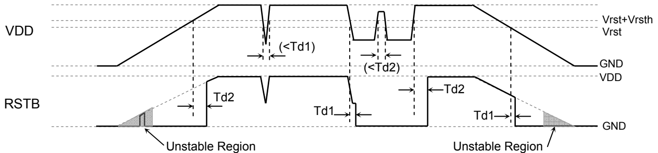
RSTB Timing Chart
