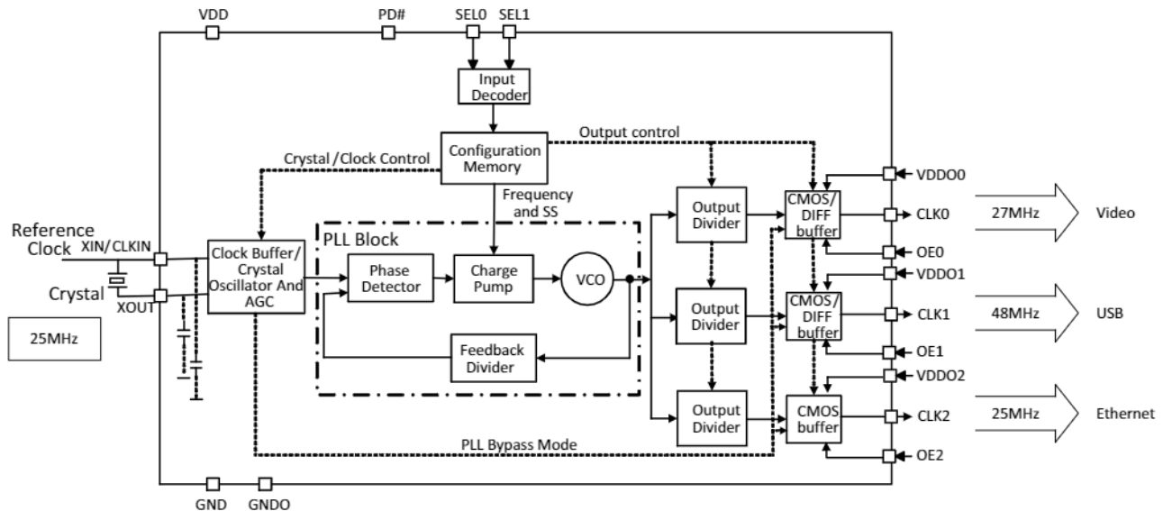
Figure 19. Application as Clock Generator
