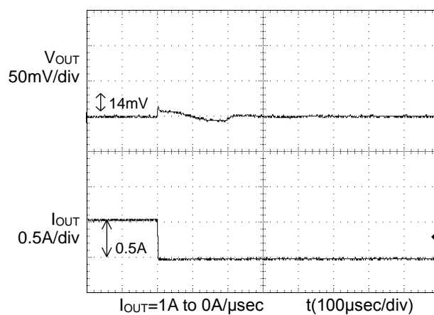
Figure 4. Transient Response (0.5 to 0A) C_{OUT}=100\mu F , C_{FB}=1000pF
