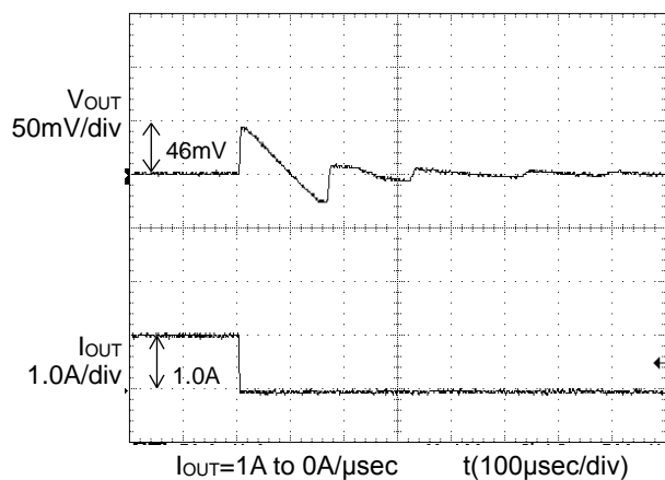
Figure 11. Transient Response (1.0A to 0A) C_{OUT}=47\mu F , C_{FB}=1000pF
