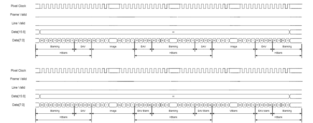
Figure 17: CCIR656 (Progressive) Output
