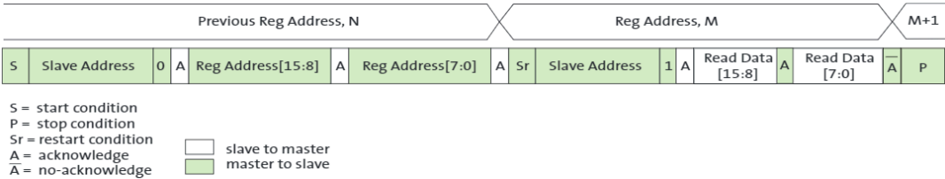
Figure 22: Single READ from Random Location
