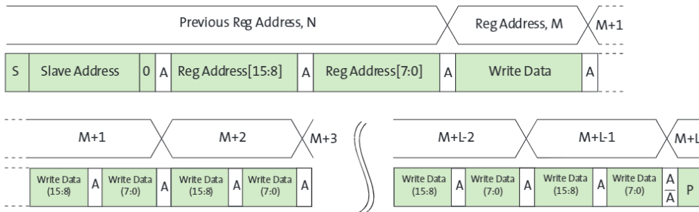
Figure 27: Sequential WRITE, Start at Random Location
