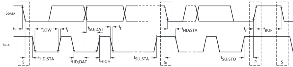
Figure 31: Master Two Wire Serial Bus Timing Parameters (CCIM)
