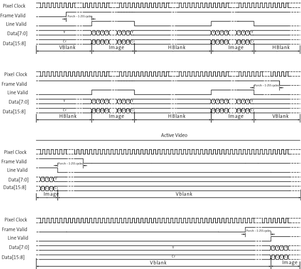
Figure 15: 16-bit YCbCr Output (YCbCr_422_16)
