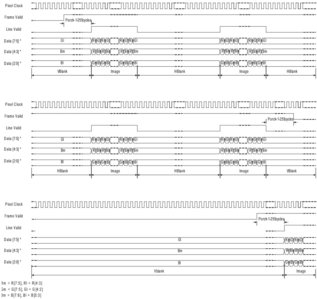
Figure 21: RGB565_8_8
