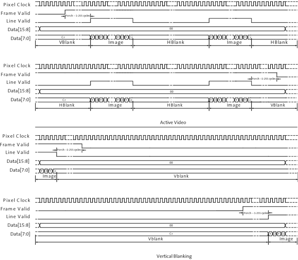
Figure 13: 8-bit YCbCr Output (YCbCr_422_8_8)
