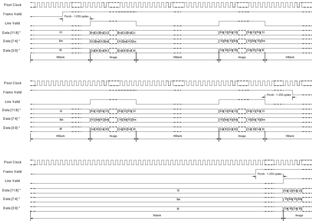
Figure 19: 12+12-bit RGB888 Output
