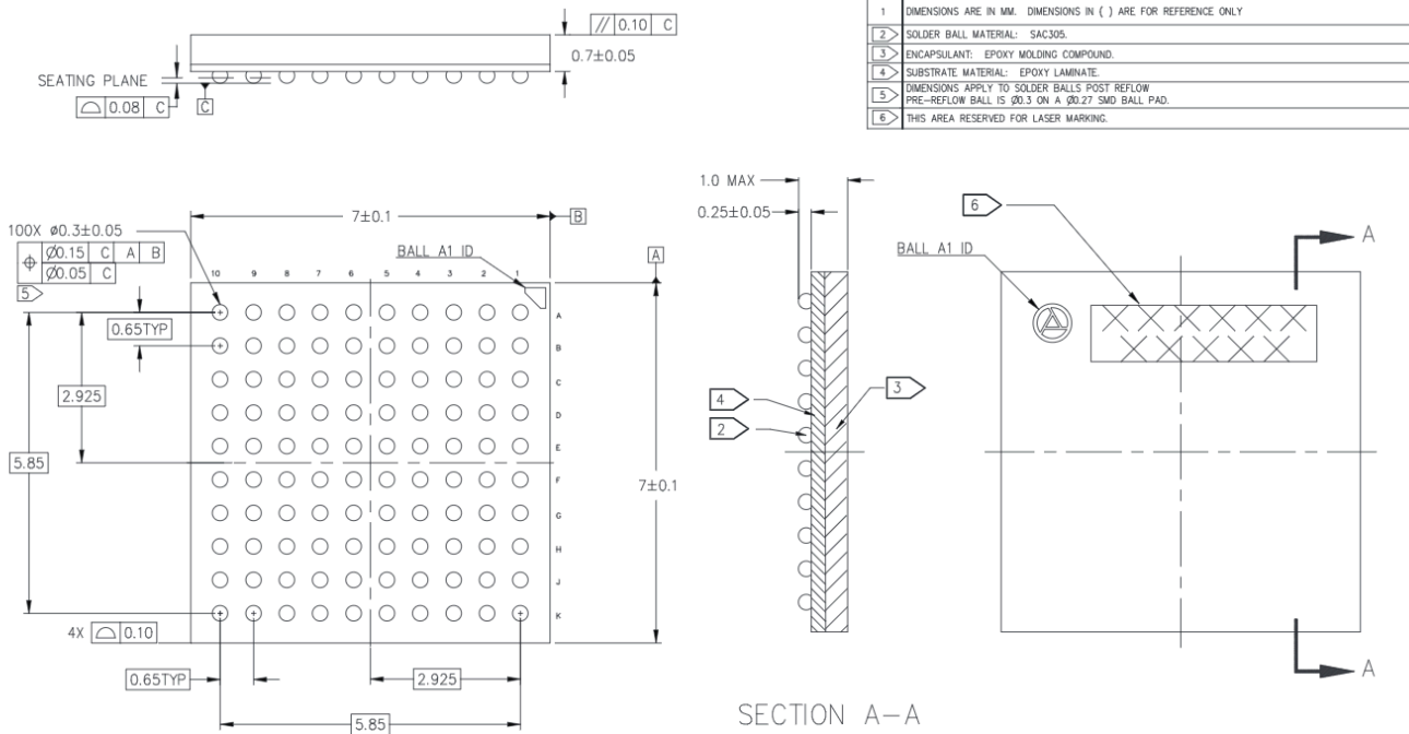
Figure 32: Package Diagram
