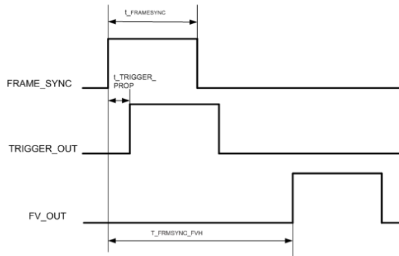
Figure 29: Frame_Sync Diagram
