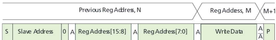
Figure 26: Single WRITE to Random Location
