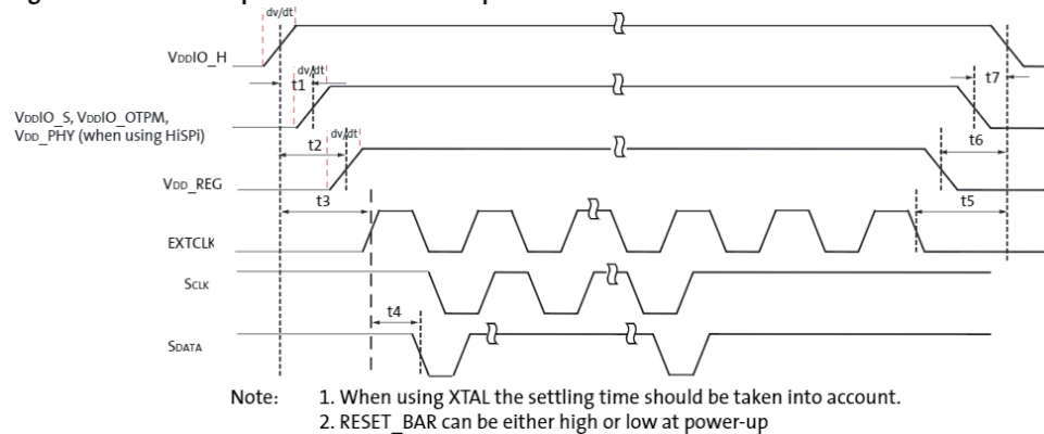
Figure 5: Power-Up and Power-Down Sequence
