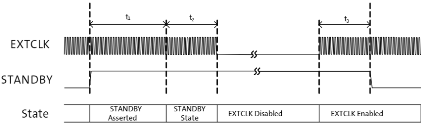
Figure 7: Hard Standby Operation
