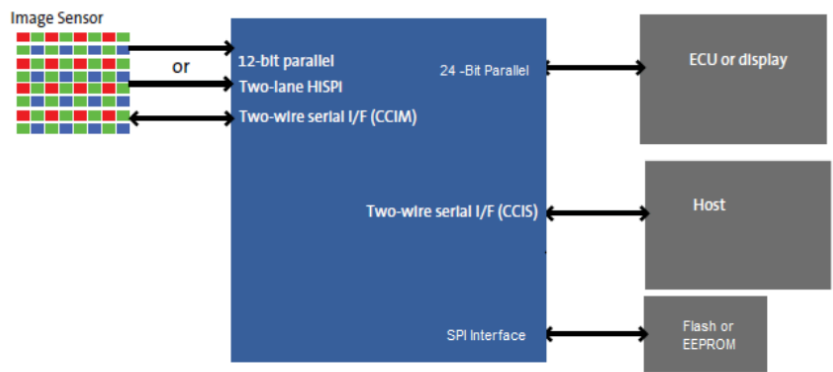
Figure 1: AP0202AT Connectivity
