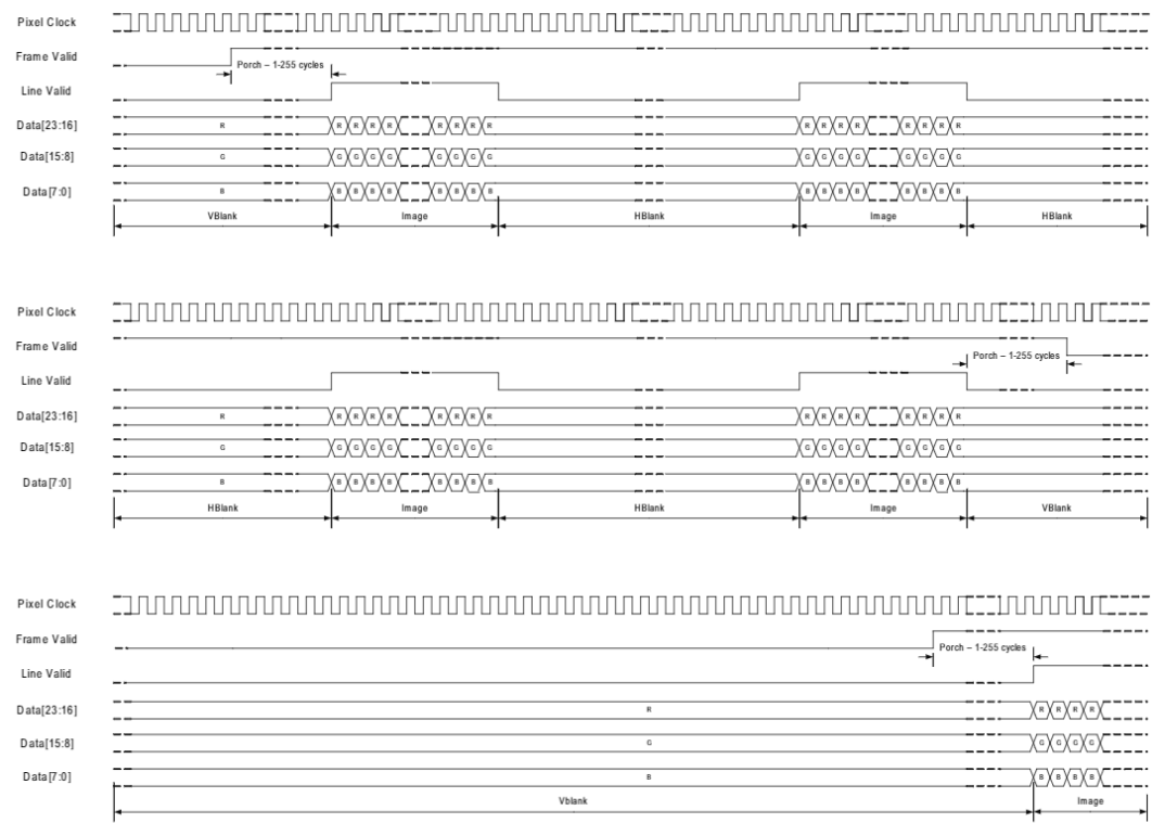
Figure 18: 24-bit RGB888 Output
