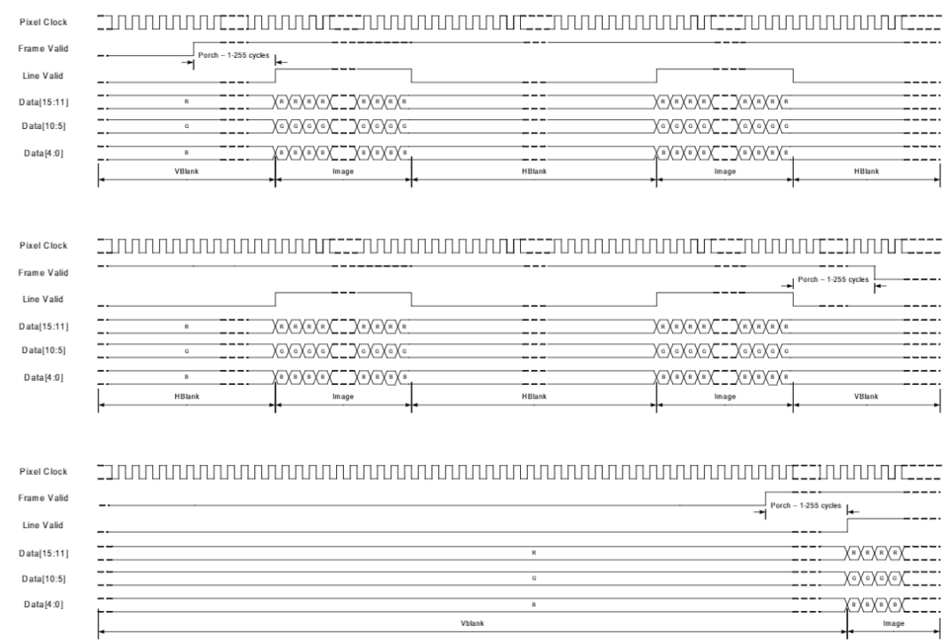
Figure 20: RGB565_16
