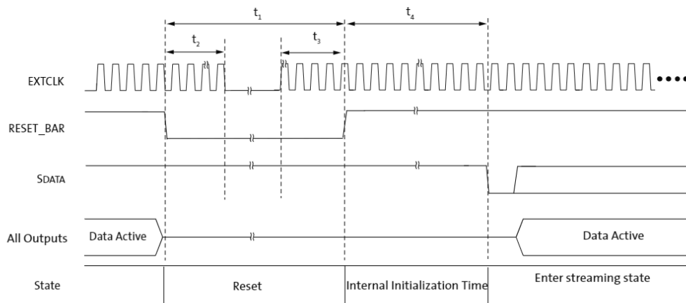
Figure 6: Hard Reset Operation
