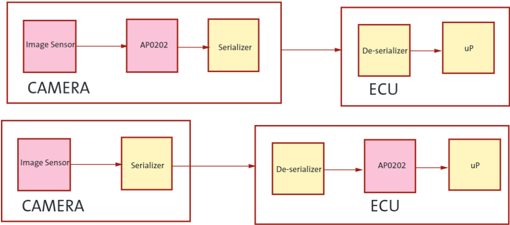
Figure 2: Examples AP0202AT Connectivity
