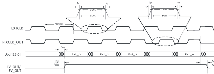
Figure 28: I/O Timing Diagram
