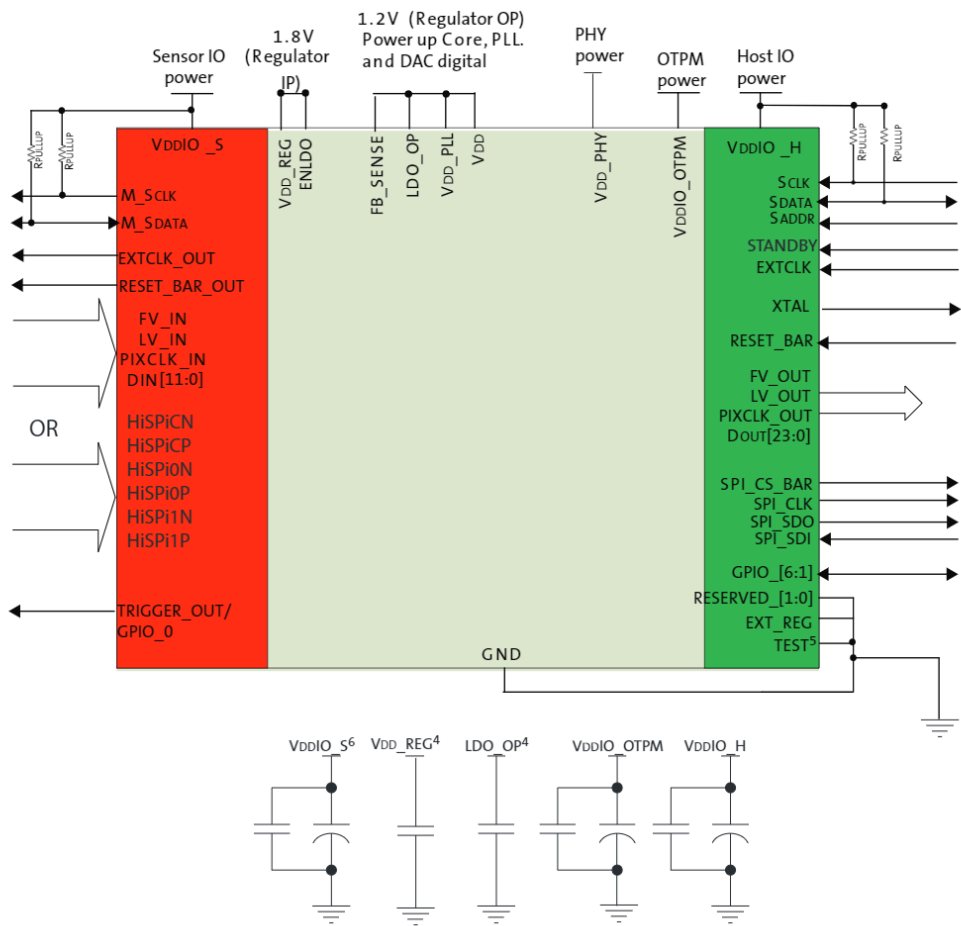
Figure 3: Typical Parallel Configuration - Legacy Mode
