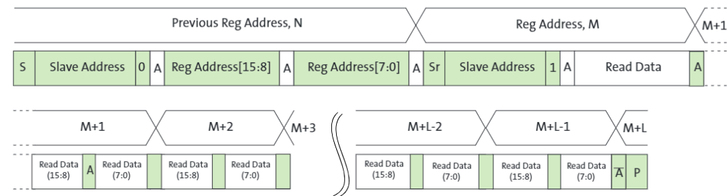
Figure 24: Sequential READ, Start from Random Location
