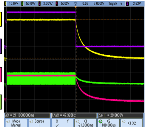
Figure 34. NCP4060A entering OTP
