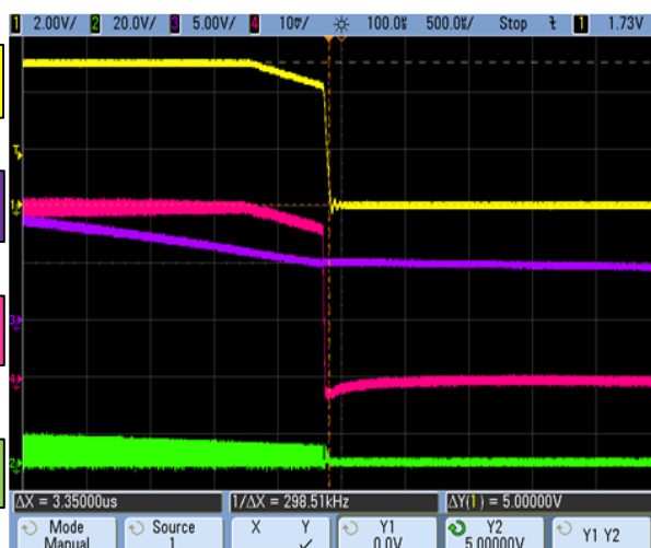
Figure 24. Shut-Down Transition at 6A Load
