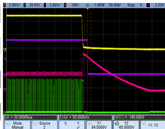
Figure 30. Short Circuit Test at 6A Load
