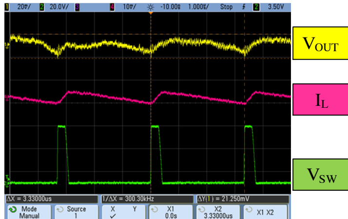
Figure 19. Steady State Operation at No Load
