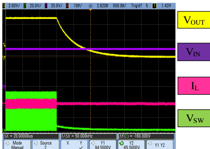
Figure 27. Shut-Down Transition at No Load (EN = Low)
