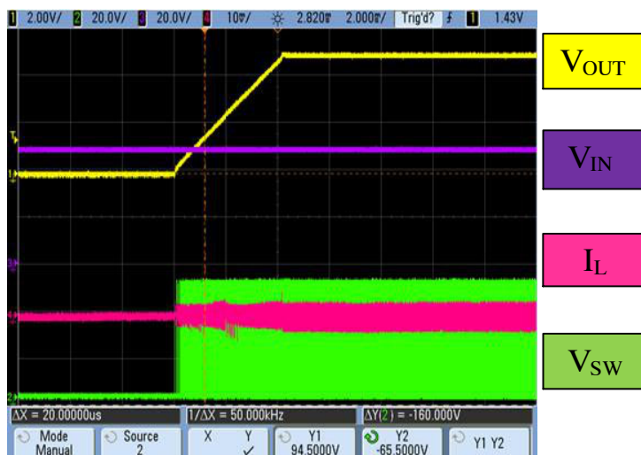
Figure 25. Start-Up Transition at No Load (EN = High)
