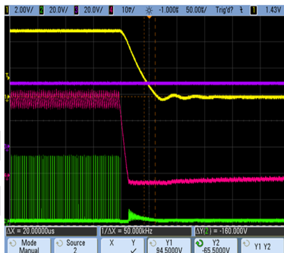
Figure 28. Shut-Down Transition at 6A Load (EN = Low)
