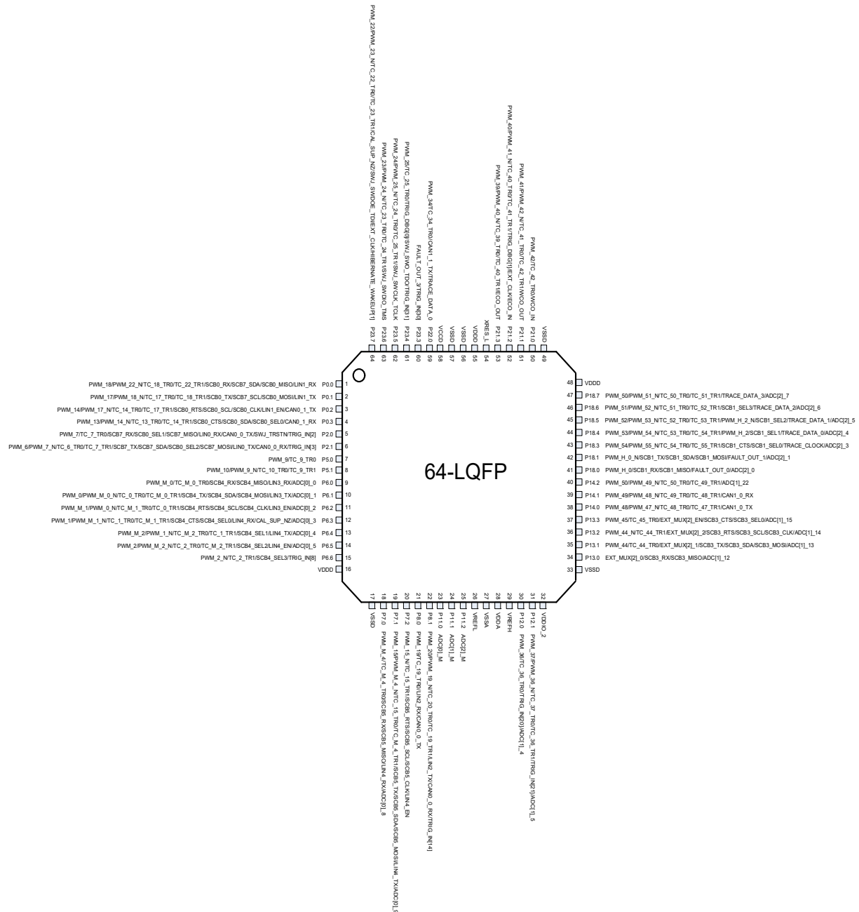
Figure 9-6.64-LQFP Pin Assignment with Alternate Functions
