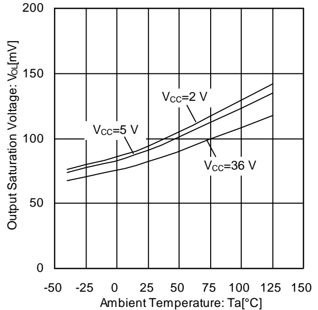
Figure 23. Output Saturation Voltage vs Ambient Temperature (I SINK =4 mA)
