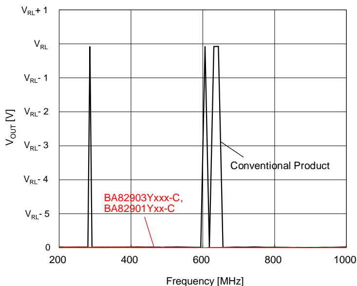
Figure 43. EMI Characteristics (L Level Output)
