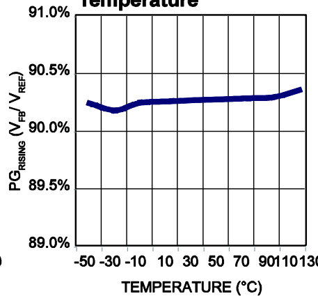
PG Rising Threshold (V FB Rising) vs. Temperature
