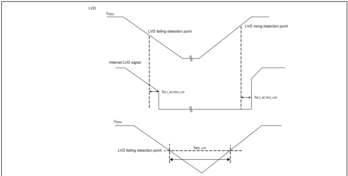
Figure 26-20 LVD specifications
