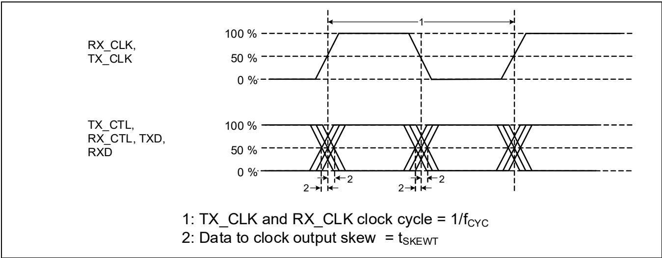
Figure 26-28 RGMII Tx timing diagram
