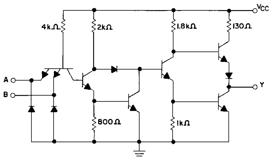
SCHEMATIC A
