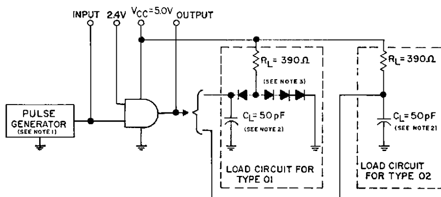
TEST CIRCUIT
