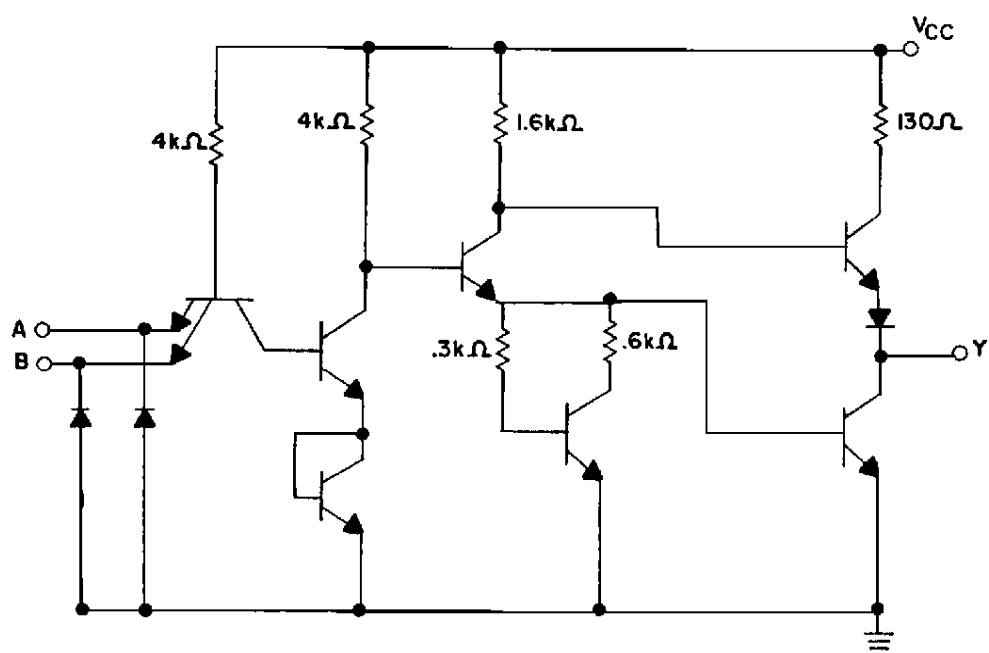
SCHEMATIC B
