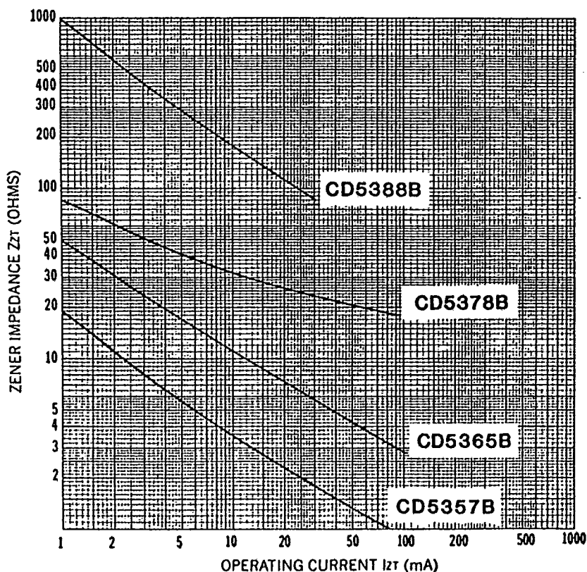
FIGURE 3 TYPICAL CHANGE OF ZENER IMPEDANCE WITH CHANGE IN OPERATING CURRENT FOR TYPES SHOWN
