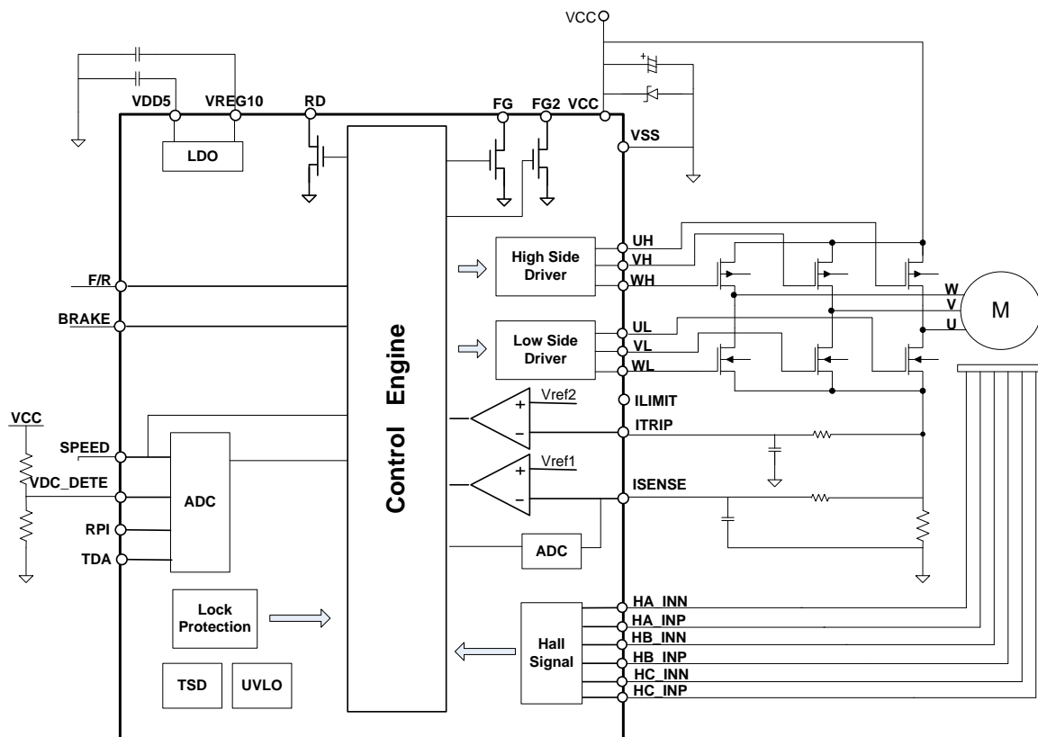
FT1128T Application Circuit
