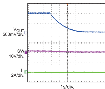
Thermal Shutdown
