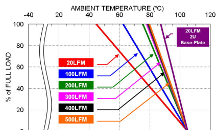
QAE60-72S05U Derating Curve (See Thermal Considerations)
