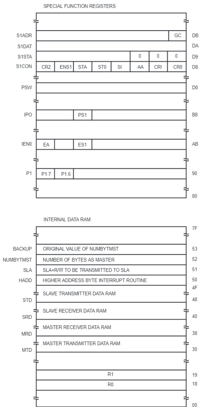
Figure 47. SIO1 Data Memory Map
