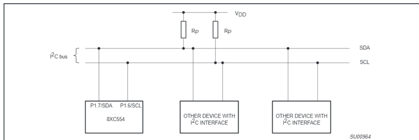
Figure 33. Typical I 2 C Bus Configuration
