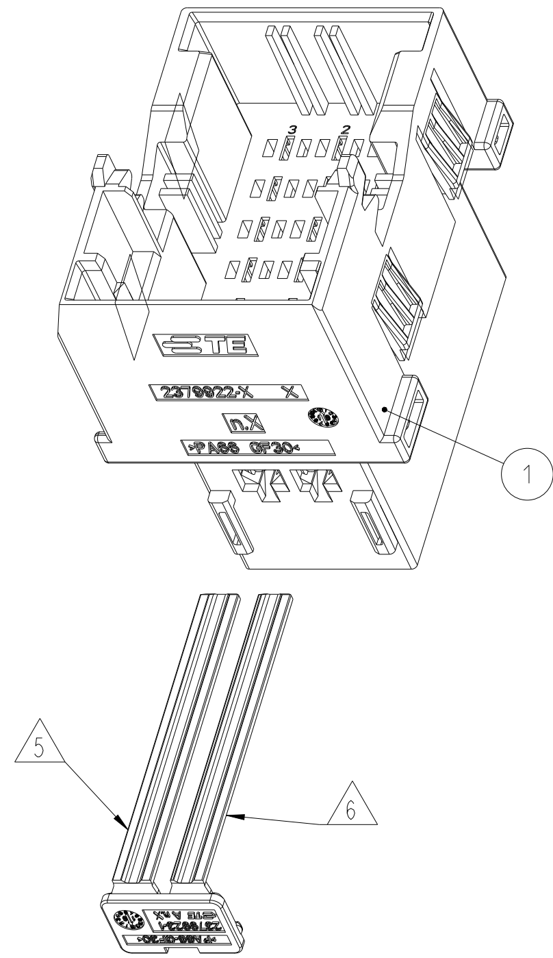
REFERENCE VIEW ASSEMBY WITH SECOND LOCK DEVICE
