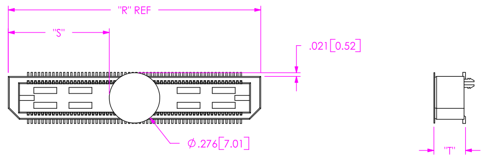
FIG. 2 -K: POLYAMIDE FILM PAD OPTION [USE K-500-300]
