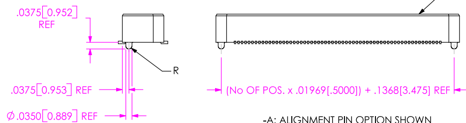
-A: ALIGNMENT PIN OPTION SHOWN
