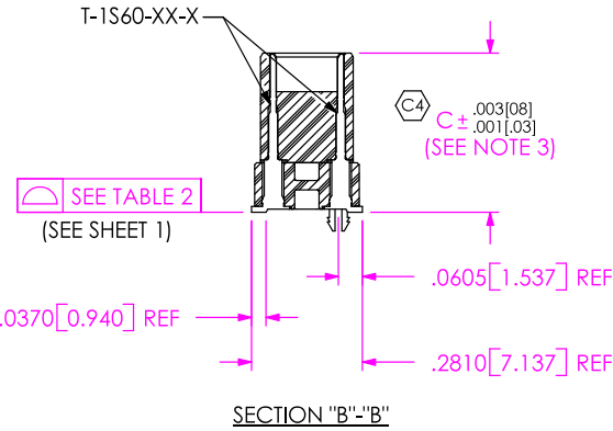
FIG. 3 BTH-060-03-X-D-LC SHOWN (STYLES -03, -04, & -09) (DIFFERENT AS SHOWN, OTHERWISE SAME AS FIG. 1)
