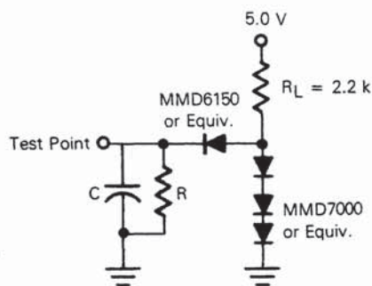
FIGURE 3 — BUS TIMING TEST LOAD
