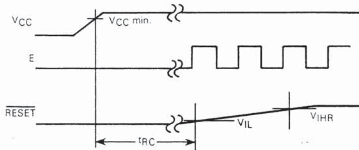
FIGURE 7 — CRYSTAL CONNECTIONS AND OSCILLATOR START UP
