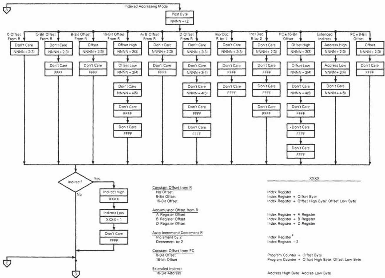
FIGURE 18 — CYCLE-BY-CYCLE PERFORMANCE (Sheet 4 of 5)
