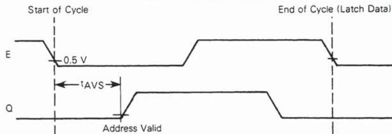
FIGURE 11 — E/Q RELATIONSHIP
