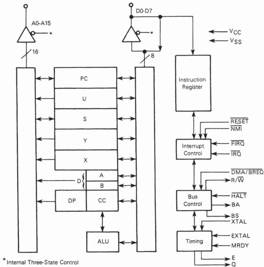
FIGURE 2 — MC6809 EXPANDED BLOCK DIAGRAM
