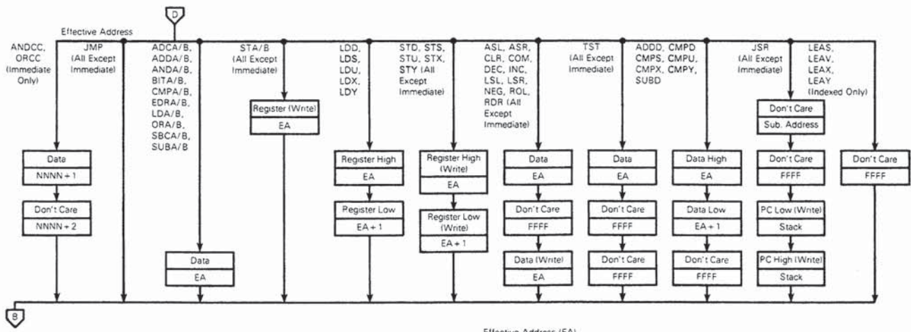
FIGURE 18 — CYCLE-BY-CYCLE PERFORMANCE (Sheet 5 of 5)
