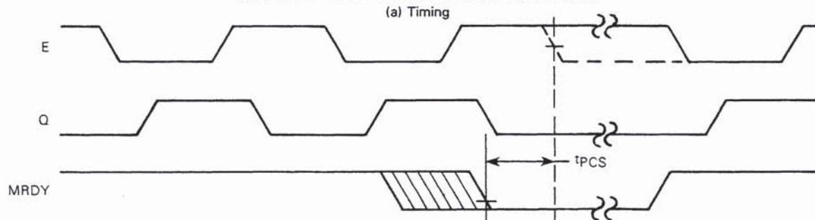
FIGURE 12 — MRDY TIMING AND SYNCHRONIZATION
