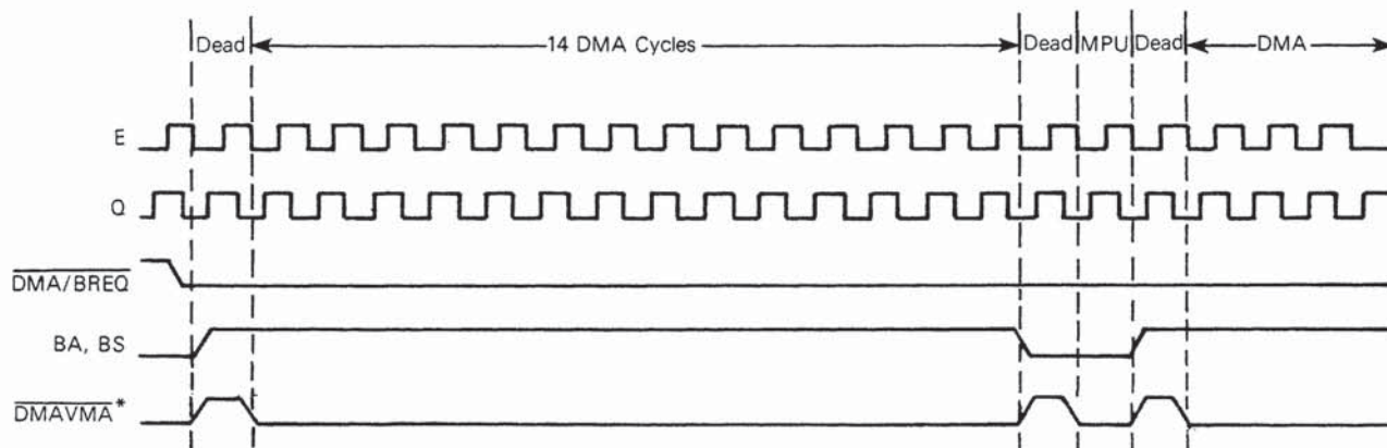
FIGURE 14 — AUTO-REFRESH DMA TIMING (>14 CYCLES) (REVERSE CYCLE STEALING)
