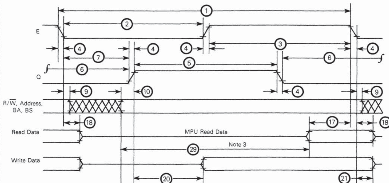
FIGURE 1 — BUS TIMING
