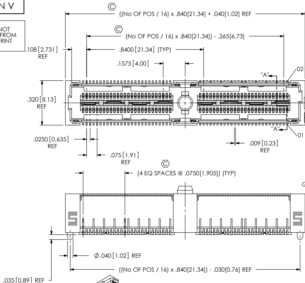
FIG 1 QFSS-032-04.25-X-D-DP-A SHOWN
