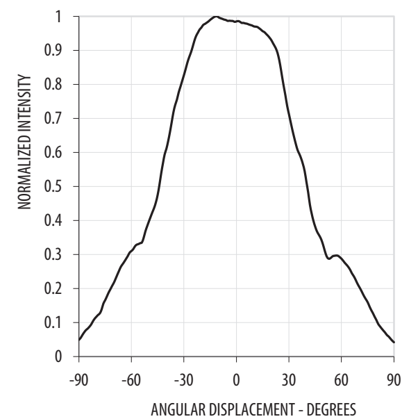
Figure 5: Radiation Pattern
