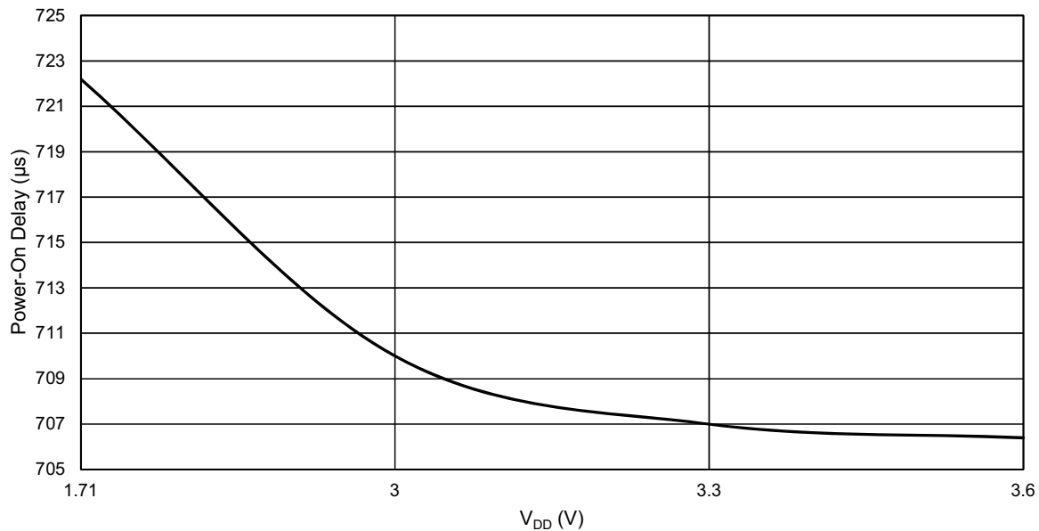
Figure 102: LF Oscillator Maximum Power-On Delay vs. V_{DD} at T = 25^{\circ}\text{C} , \text{OSC} = 1.73 \text{ kHz}
