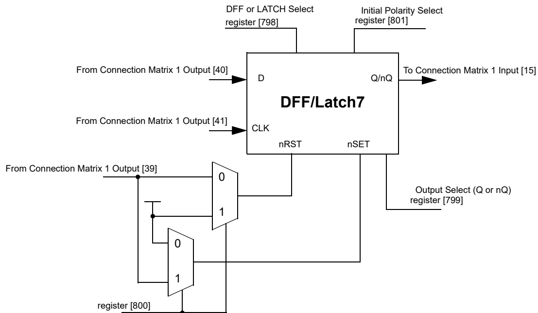
Figure 54: DFF/Latch7
