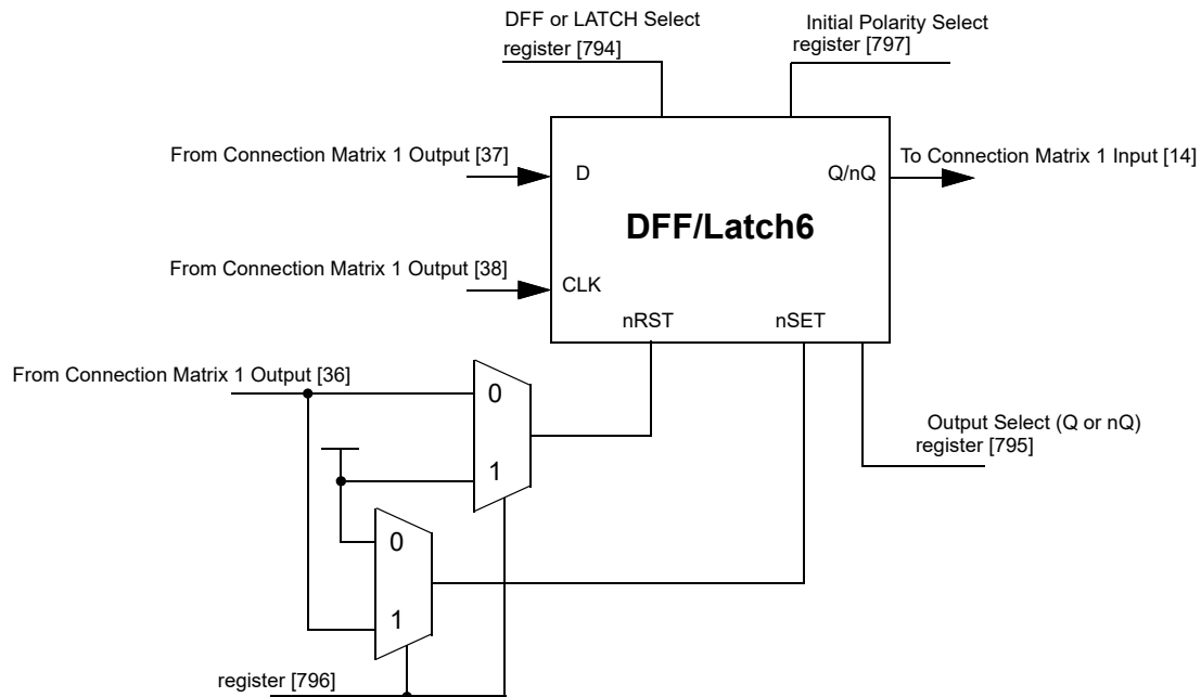
Figure 53: DFF/Latch6
