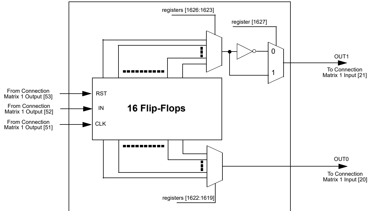
Figure 92: Pipe Delay 1
