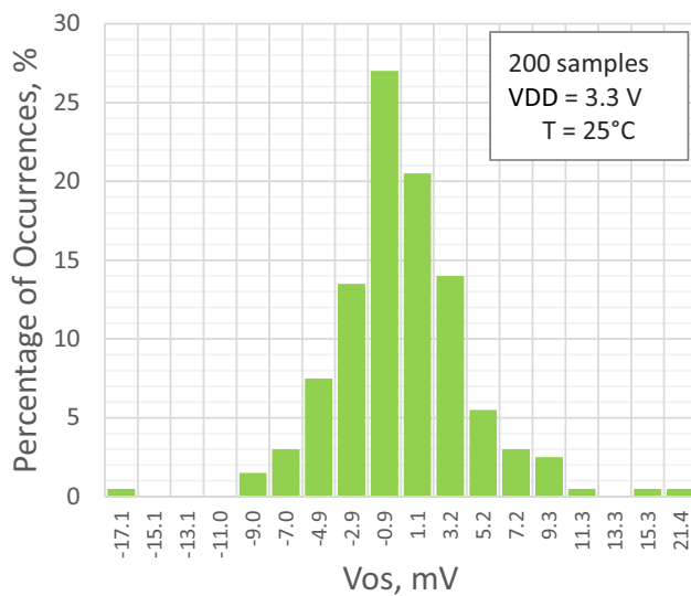
Figure 17: PGA Input Offset Distribution, Single-Ended Mode, G = 0.5
