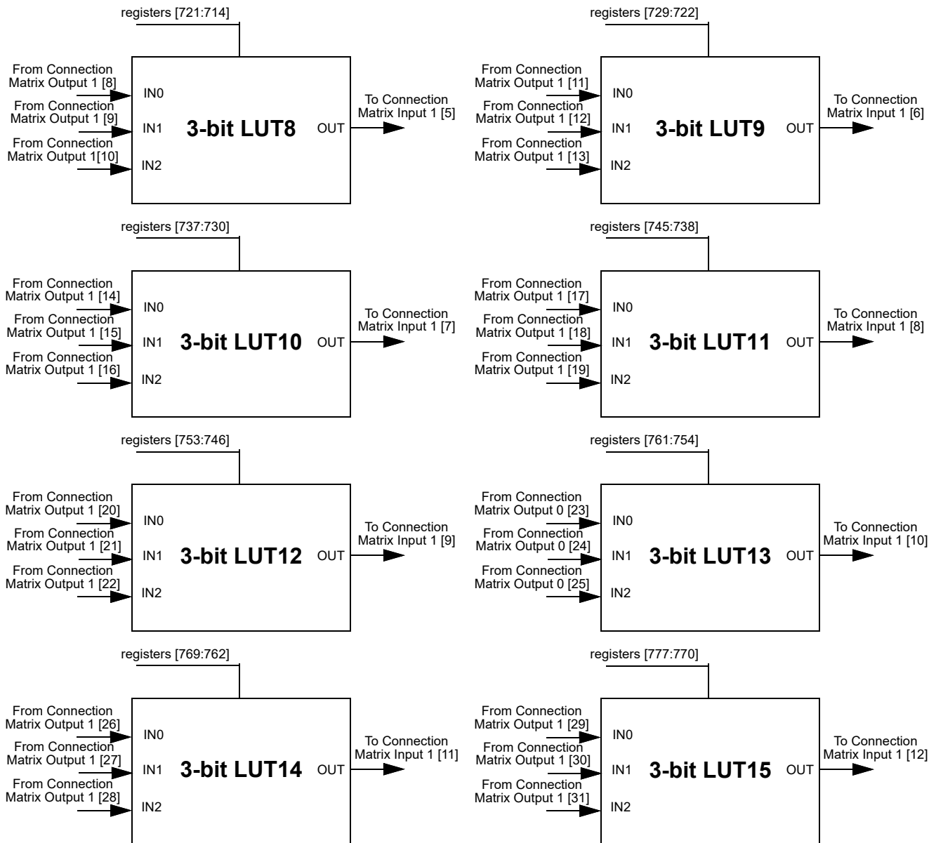
Figure 33: 3-bit LUTs
