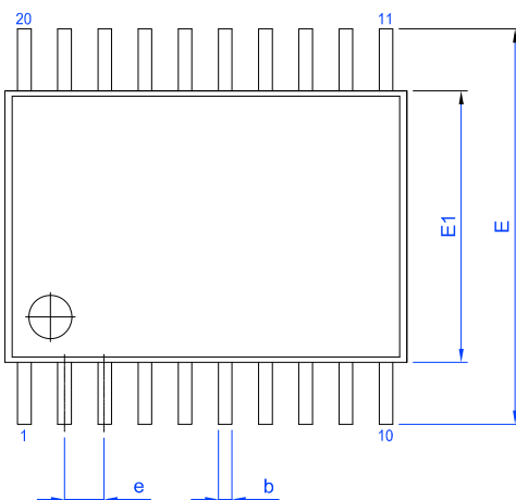
Marking View
