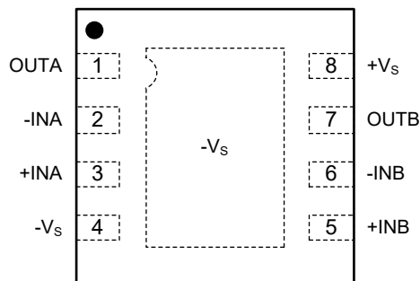
TDFN-3x3-8L
