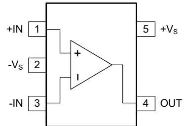
SC70-5
