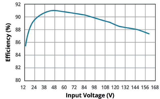
EFFICIENCY VS INPUT VOLTAGE (25°C, FULL LOAD) PVQ100W-072-S54-D
