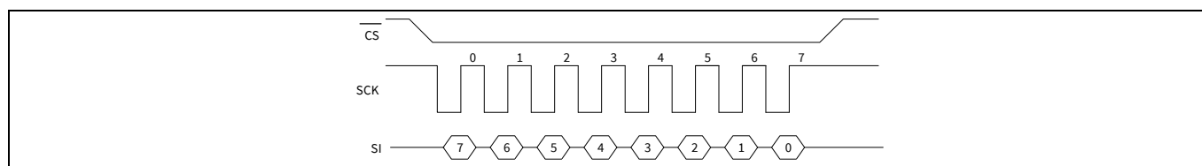
Figure 6 SPI mode 3
