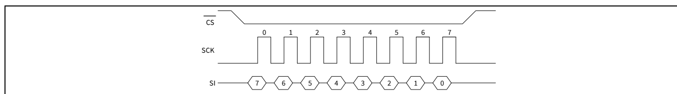
Figure 5 SPI mode 0
