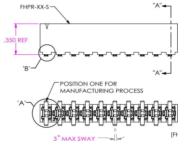
FIG 1 [FHP-10-02-X-S SHOWN]
