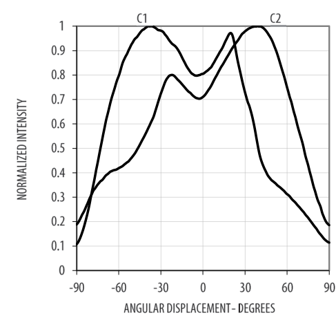
Figure 4: Radiation Pattern
