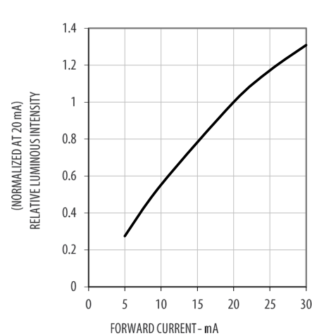
Figure 3: Relative Intensity vs. Forward Current
