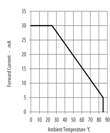
Figure 5: Derating Curve
