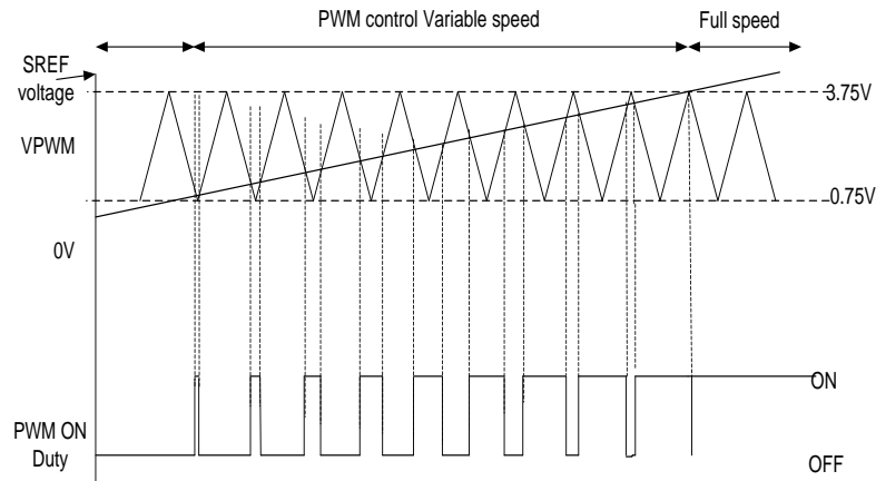
Figure 3 Rotation Speed Control Chart
