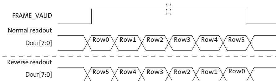
Figure 13: Six Rows in Normal and Row Mirror Readout Mode
