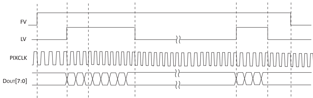
Figure 28: JPEG Continuous Data Output
