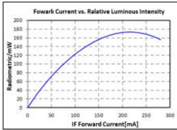
Fig.1-Relative Luminous Intensity vs. Forward Current
