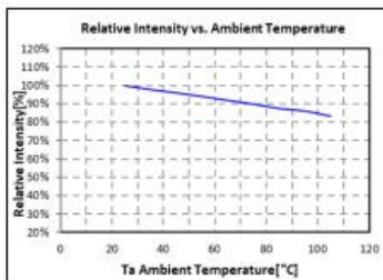
Fig.3-Relative Intensity (@60mA) vs. Ambient Temperature
