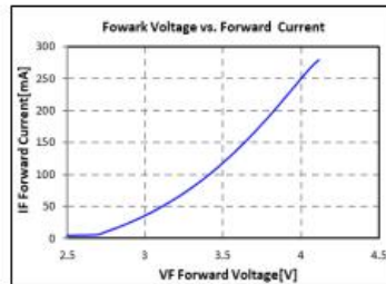
Fig.2-Forward Current vs. Forward Voltage
