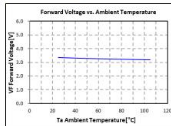
Fig.4-Forward Voltage (@60mA) vs. Ambient Temperature
