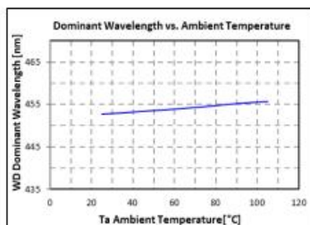
Fig.5- Dominant Wavelength (@60mA) vs. Ambient Temperature
