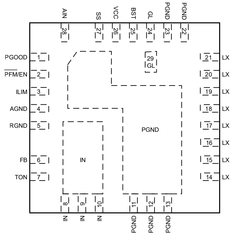
AOZ2388QI 28-pin 5mm x 5mm QFN
