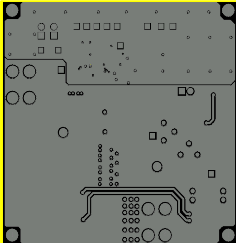
Figure 26. Evaluation Board Inner Layer 1 Copper
