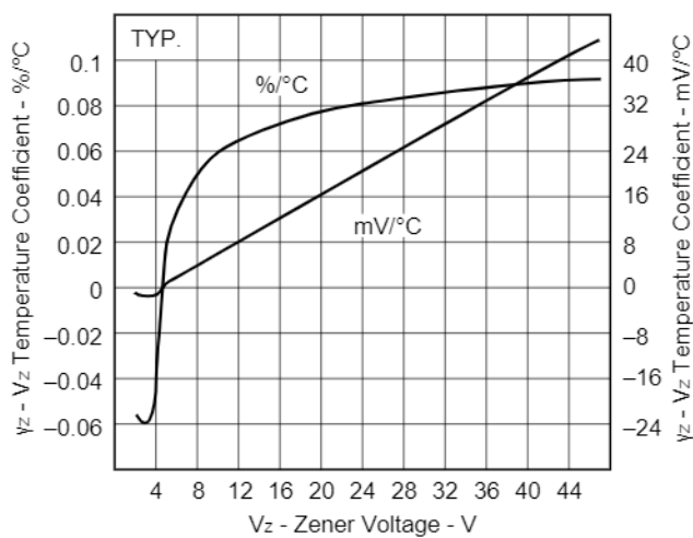
Fig. 3 V_z - V_z CHARACTERISTICS
