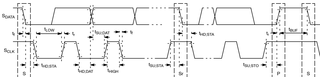
Figure 6. Two-Wire Serial Bus Timing Parameters
