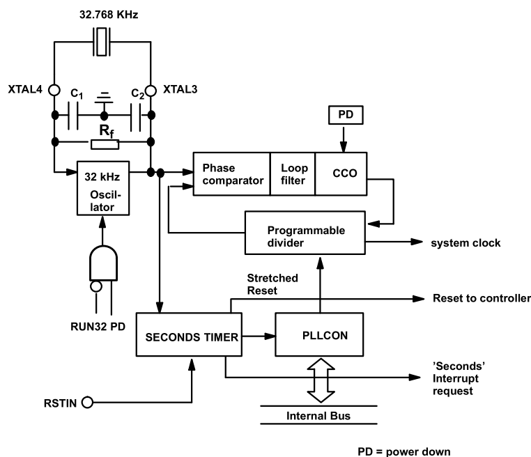
Figure 45. Block diagram PLL
