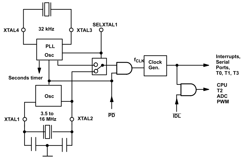
Figure 40. Idle and Power Down Hardware for Clock Generation
