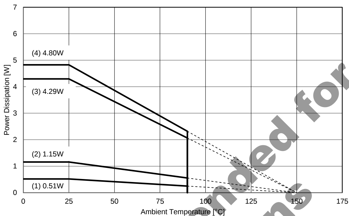
Figure 32. Power dissipation
