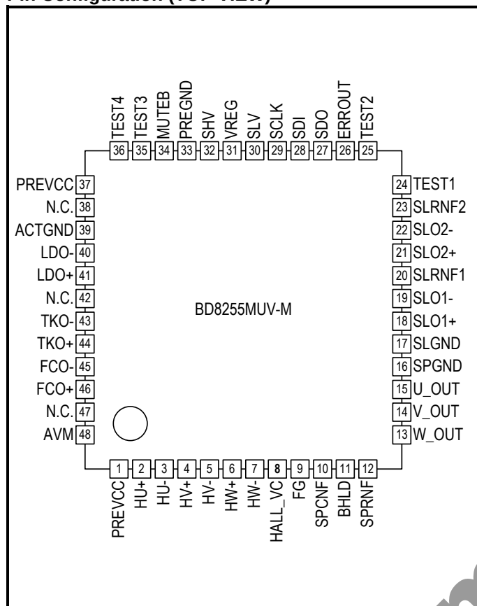
Figure 2. Pin configuration
