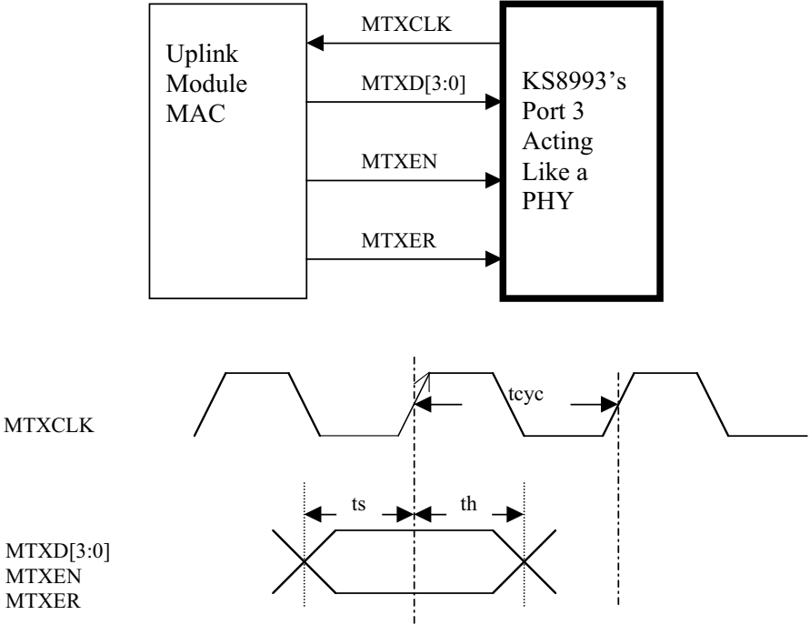
Figure 5. Reverse MII Timing–Receive Data from MII
