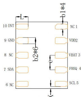
Package Bottom View
