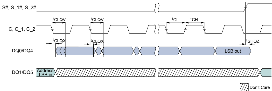
Figure 54: Output Timing
