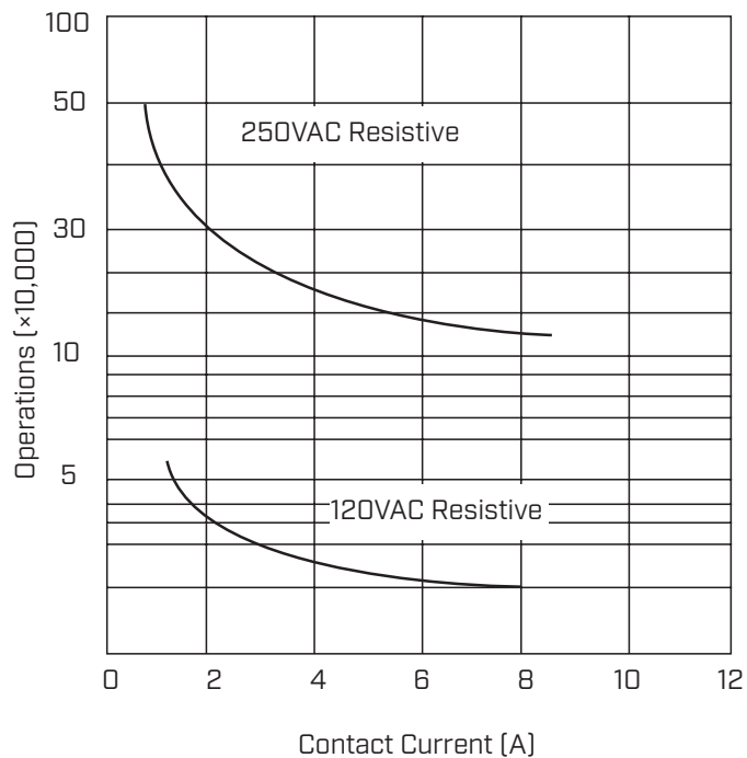
Life Curve
