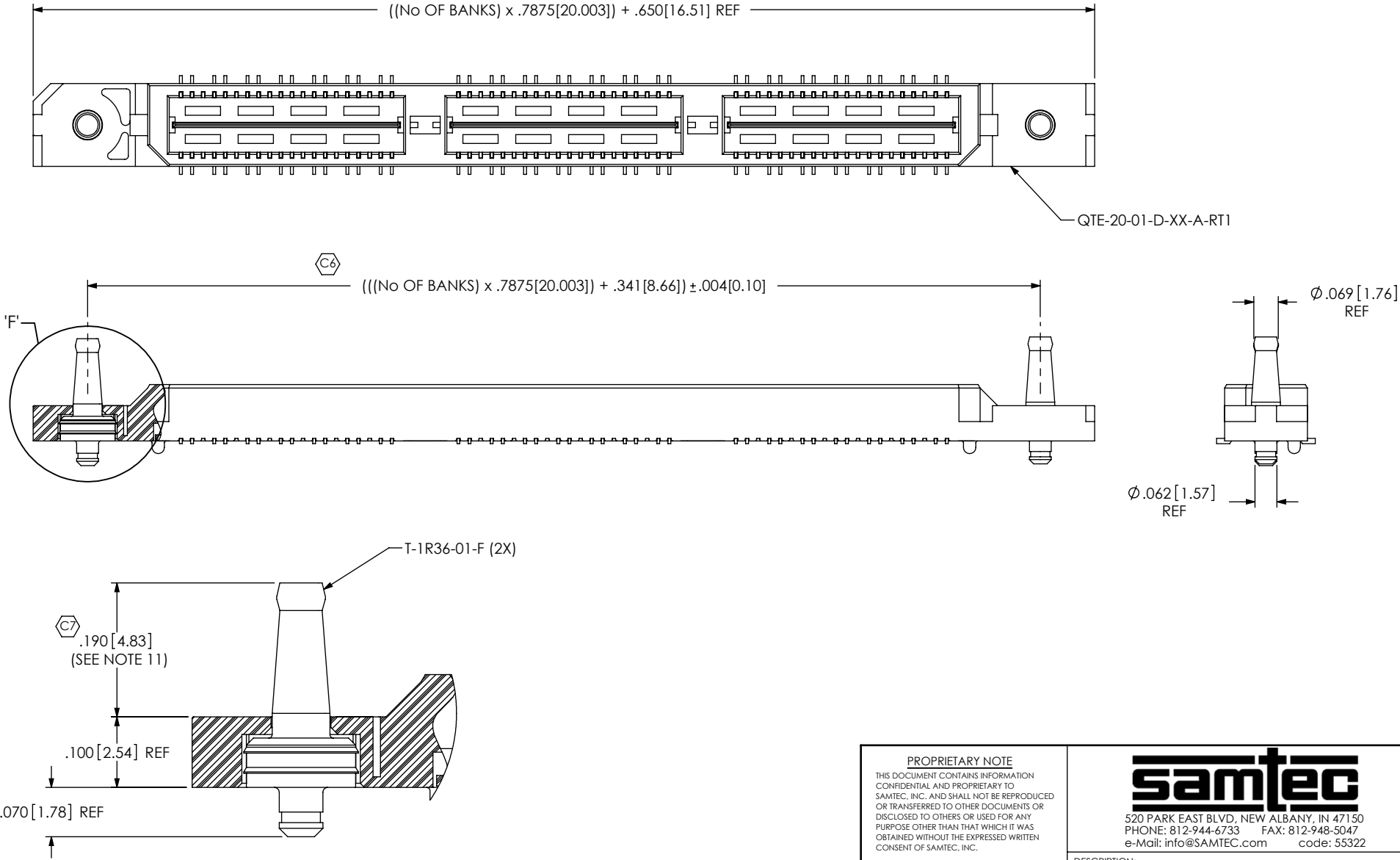
DETAIL 'F' SCALE 5:1
