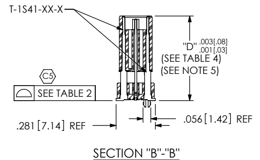
FIG. 4 QTE-042-04-X-D-DP-LC SHOWN (SAME AS FIG. 1, UNLESS OTHERWISE STATED) (STYLES -04, -05, & -06)
