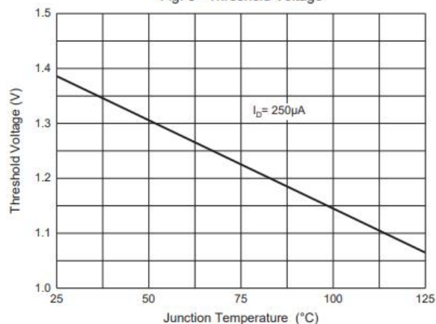
Fig. 6 - Threshold Voltage
