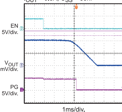
Power Good through EN Shutoff
