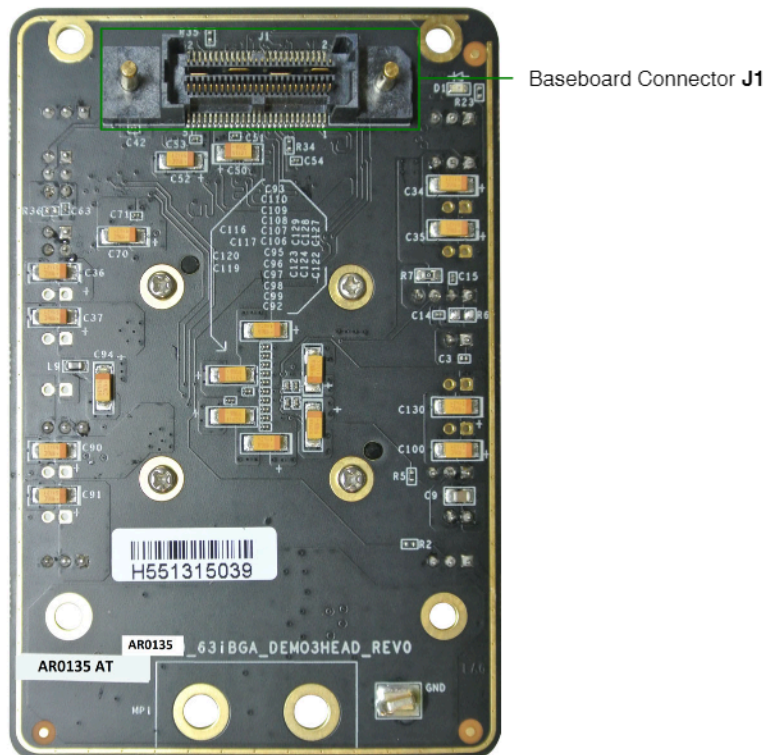
Figure 4. Bottom View of the Board – Connector
