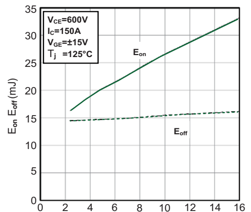
Figure 4: Switching Energy vs. Gate Resistor for IGBT Inverter
