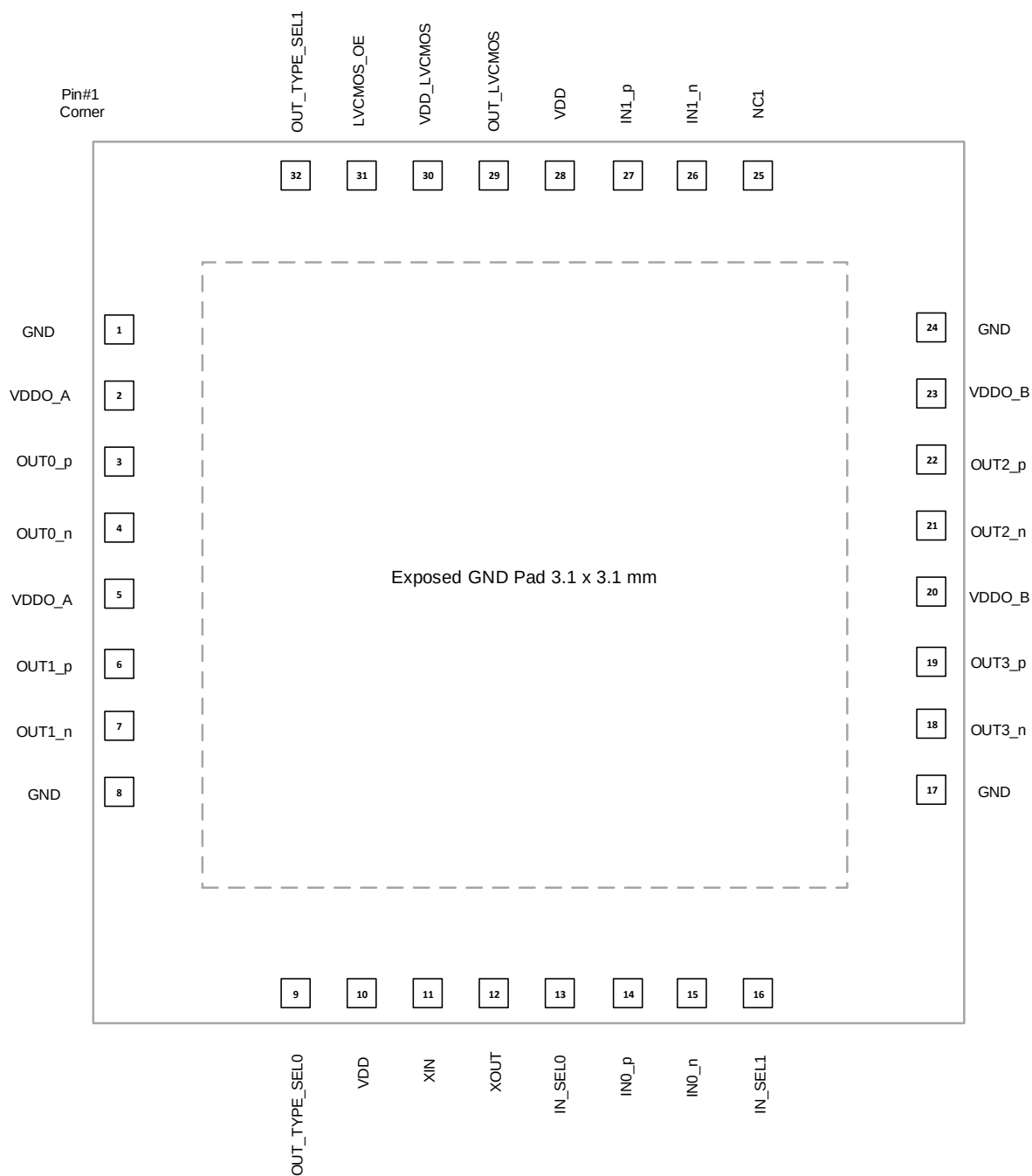
Figure 2. Pin Diagram
